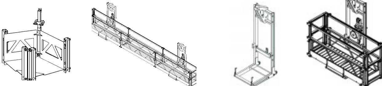
Moveable Stirrup, Adjustable Corner 1, 2, & 3 Meter Work Cages
